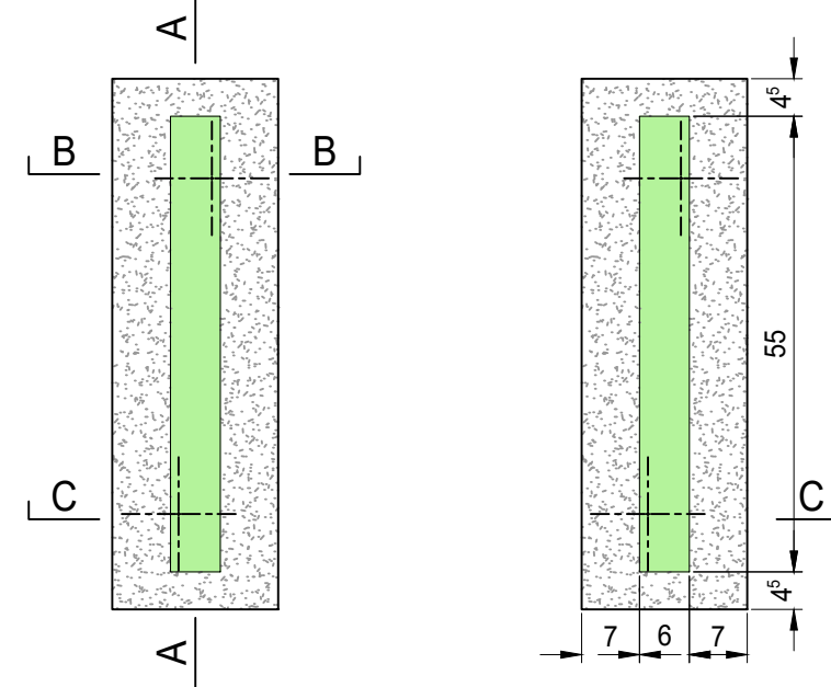
Implantation pied
